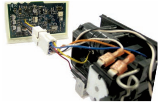
Figure 4. Connect Harness
