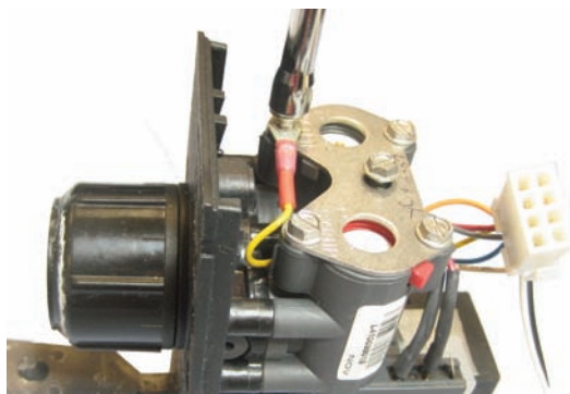
Figure 2. Yellow Wire
