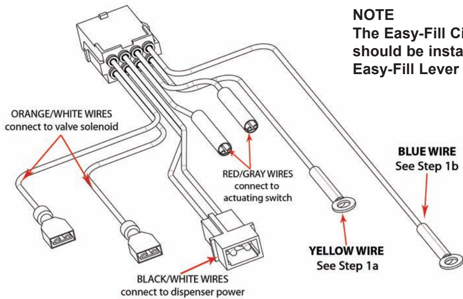
Fig 1. Connection Diagram
